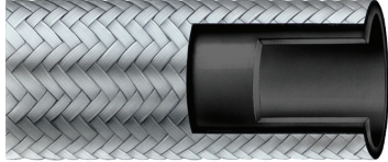
Smoothbore Black Conductive PTFE Lined Hose with Braided Stainless Steel Cover
